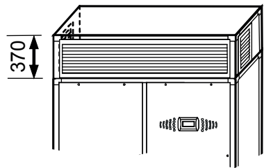
1 Discharge air plenum shows as 3 way, also available is front discharge only
