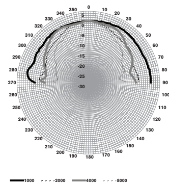
LC1-WM06E8 Polar diagrams
