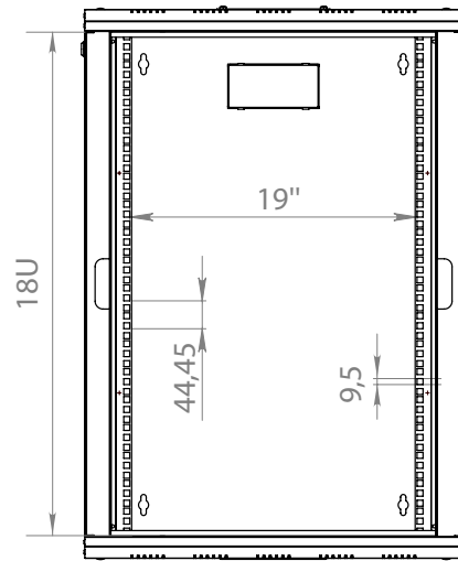
FRONT VIEW WITHOUT COVER
