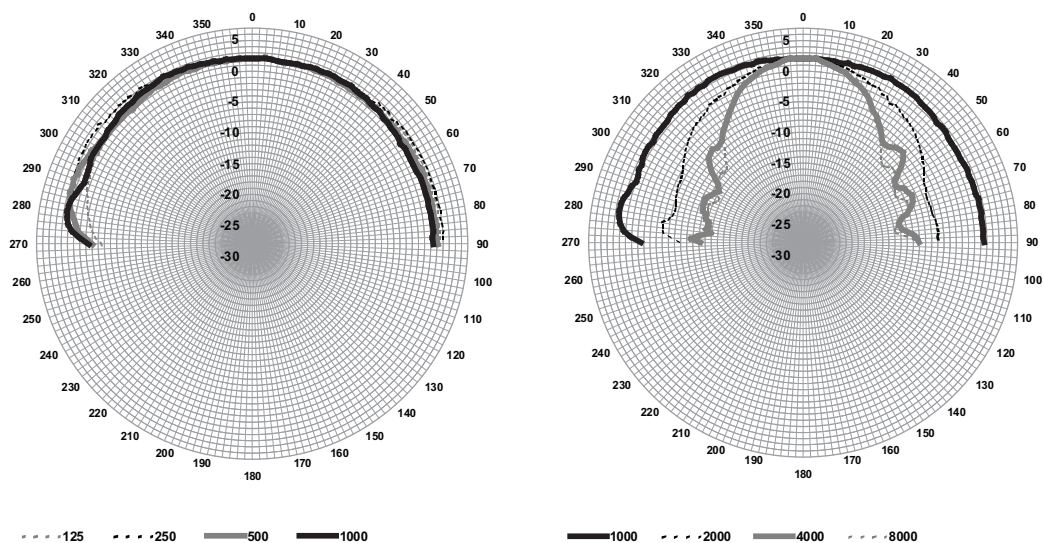
Polar diagrams
