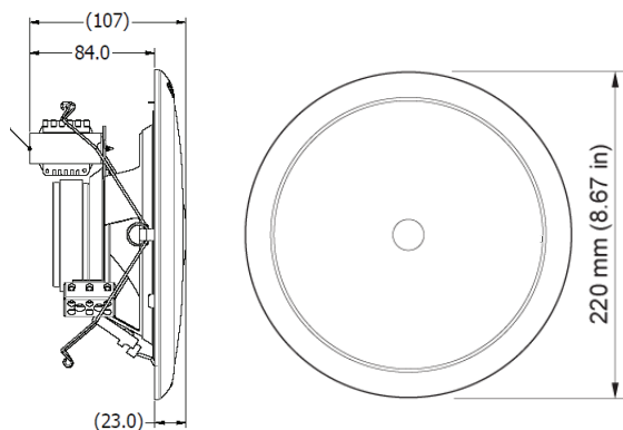
Figure 3.13: Dimensions
