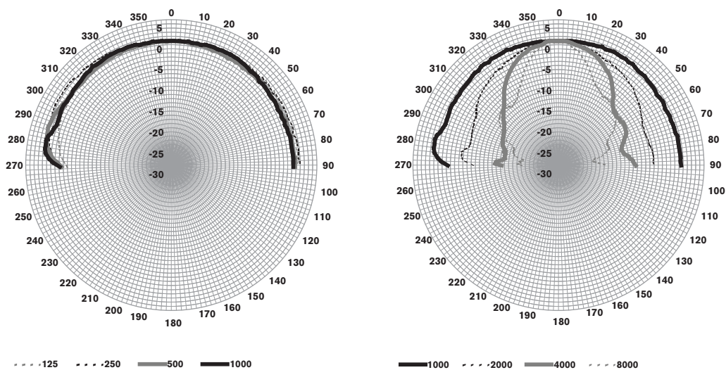
Polar diagrams
