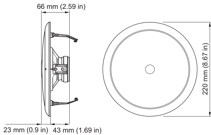
Figure 3.4: Dimensions
