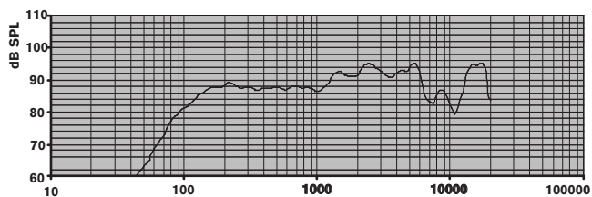
Figure 3.3: Frequency response
