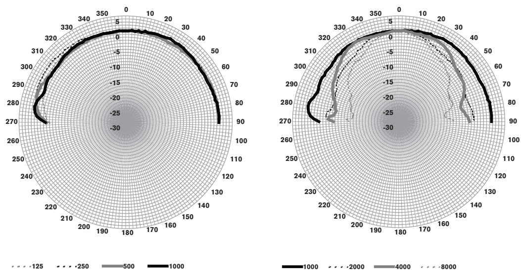
Polar diagrams
