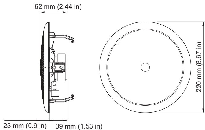
Figure 3.7: Dimensions
