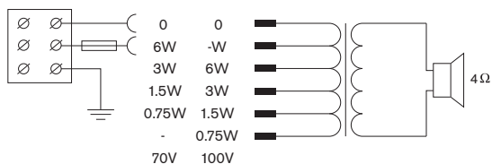
Figure 3.2: Circuit diagram
