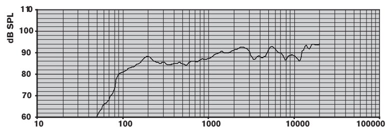
Figure 3.6: Frequency response
