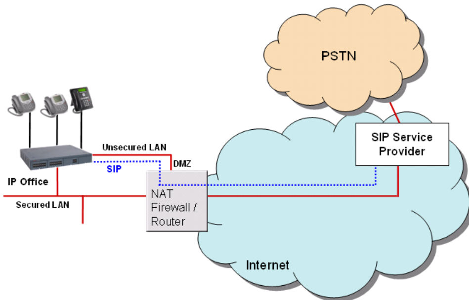
Figure : 3. Connection to ITSP over NAT using third-party STUN servers
