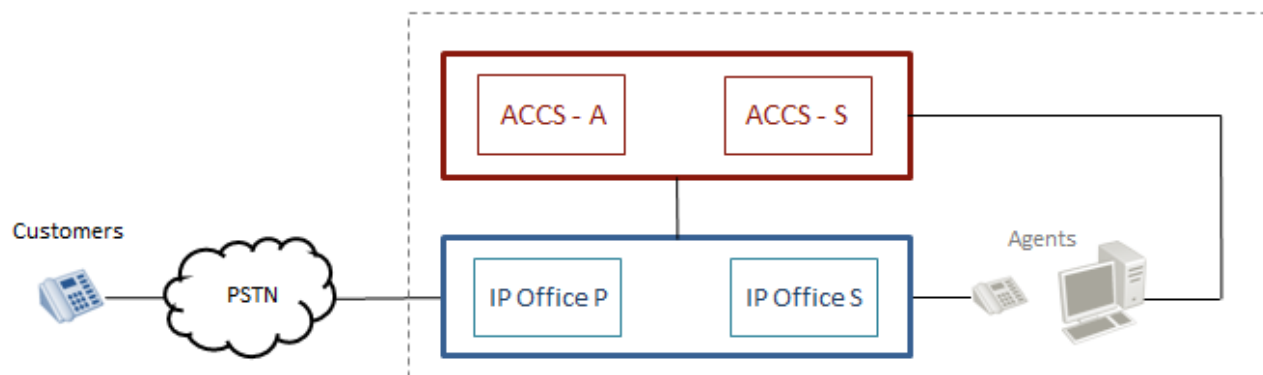
Figure : 1. Avaya Contact Center Select Business Continuity with IP Office resilience
