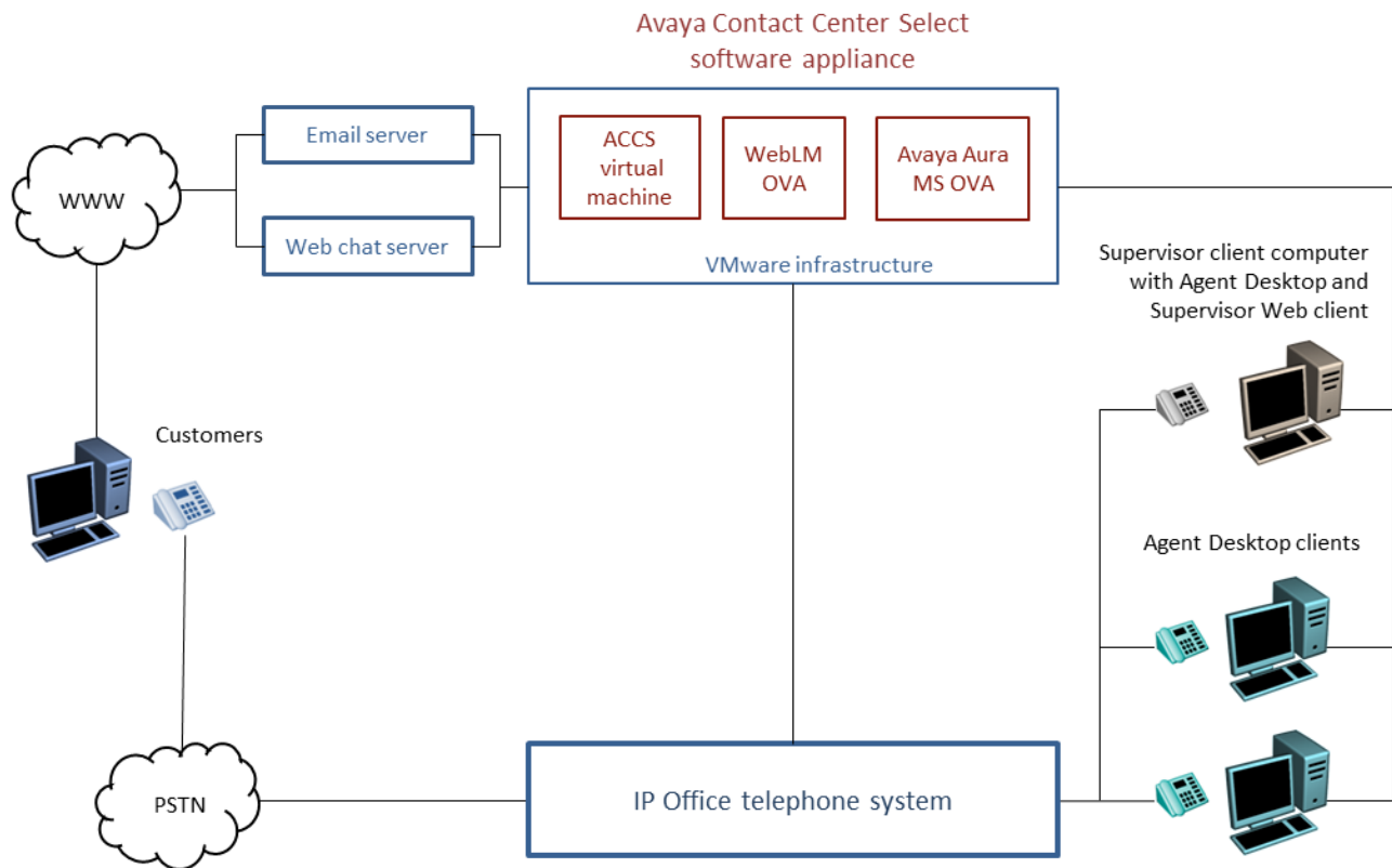
Figure : 1. Typical Avaya Contact Center Select and VMware solution
