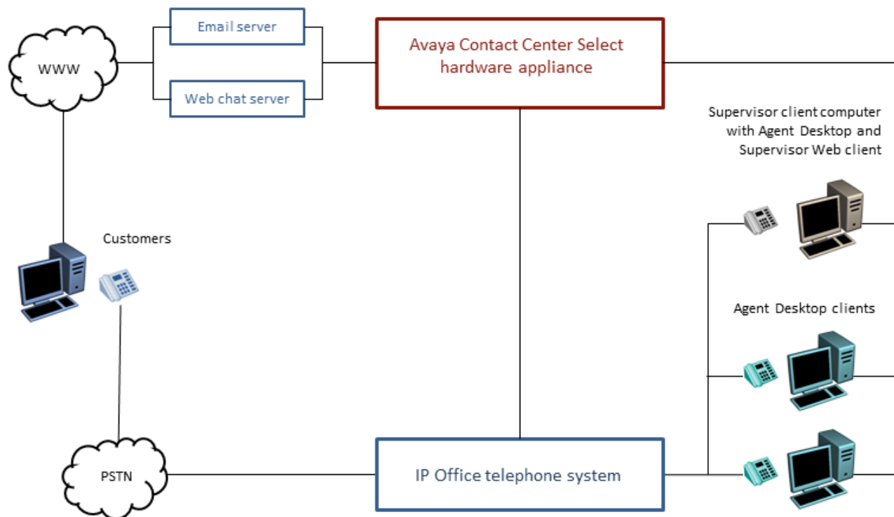
Figure : 1. Typical Avaya Contact Center Select hardware appliance solution
