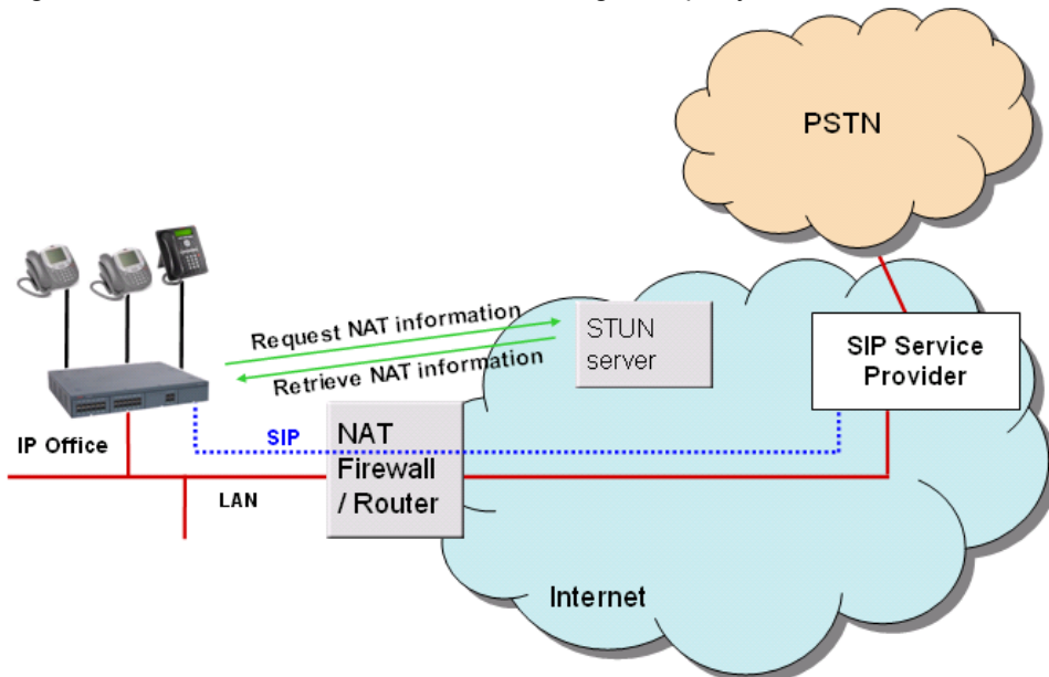
Figure : 4. Connection to ITSP through router with ALG to resolves NAT issues
